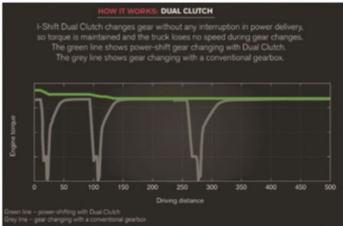
Example of dual clutch transmission
